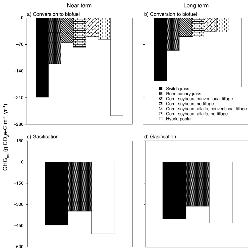
FIG. 4. Net greenhouse-gas ( \text{GHG}_{\text{net}} ) emissions from different bioenergy cropping systems with conversion to ethanol or biodiesel (a, b) or gasification of biomass (c, d). Near-term \text{GHG}_{\text{net}} is the sum of displaced fossil fuel, net change ( \Delta ) in system C, feedstock conversion, direct and indirect \text{N}_2\text{O} emissions, fossil fuel used to produce chemical inputs, and fossil fuel used in agricultural-machinery operations. Long-term \text{GHG}_{\text{net}} is the sum in near-term \text{GHG}_{\text{net}} except \Delta system C because soils will come to equilibrium with C inputs and further soil C sequestration will not occur.
