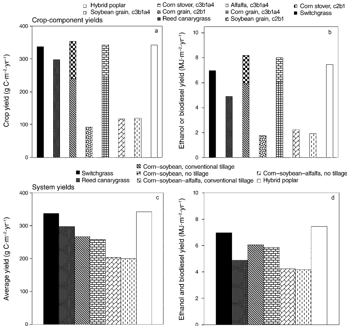
Fig. 1. Crop and fuel yield from bioenergy cropping systems. Yields are expressed either as crop component (a, b) or system (c, d) yields. Corn yields assumed that only 50% of the corn stover (leaves and stalks) was harvested; alfalfa yields only contained stems, 50% of the total yield. (a) Component yields are presented; the 2-yr corn and 1-yr soybean (c2b1) rotation and 3-yr corn, 1-yr soybean, and 4-yr alfalfa (c3b1a4) rotation yields are from the conventional-tillage system. (b) All crop components were converted to ethanol except soybean grain, which was converted to biodiesel. (c) System yields were combined from crop rotations and annualized over the rotation cycle. (d) Crop component fuel yields of ethanol and biodiesel were combined to give system yields.
