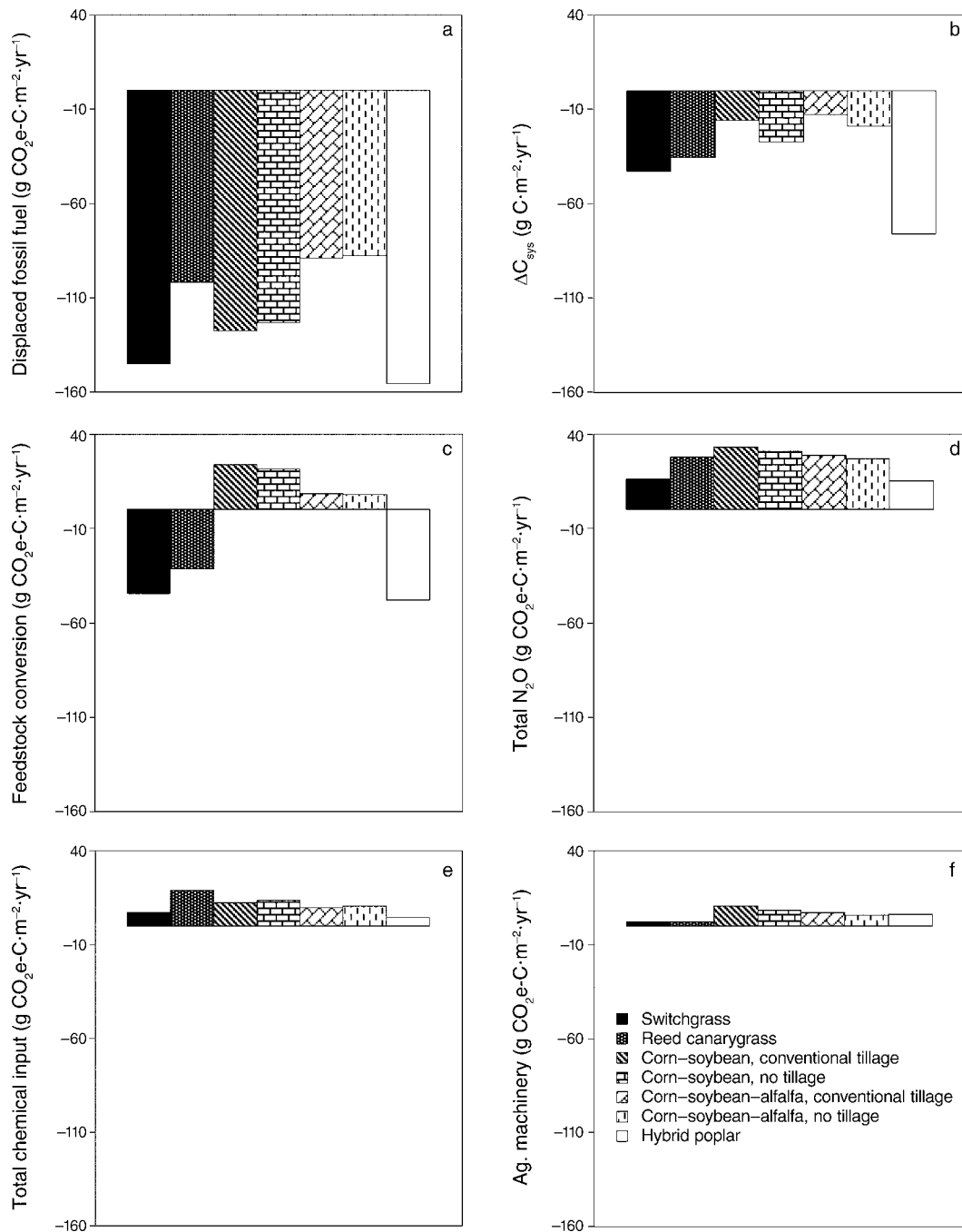
FIG. 2. Components of the net greenhouse-gas (GHG net ) profile from different bioenergy cropping systems. Displaced fossil fuel and feedstock conversion are based on displacement of gasoline and diesel and conversion of crop components to either ethanol or biodiesel. CO 2 e stands for “CO 2 equivalent”; see Table 2 note for definition.
