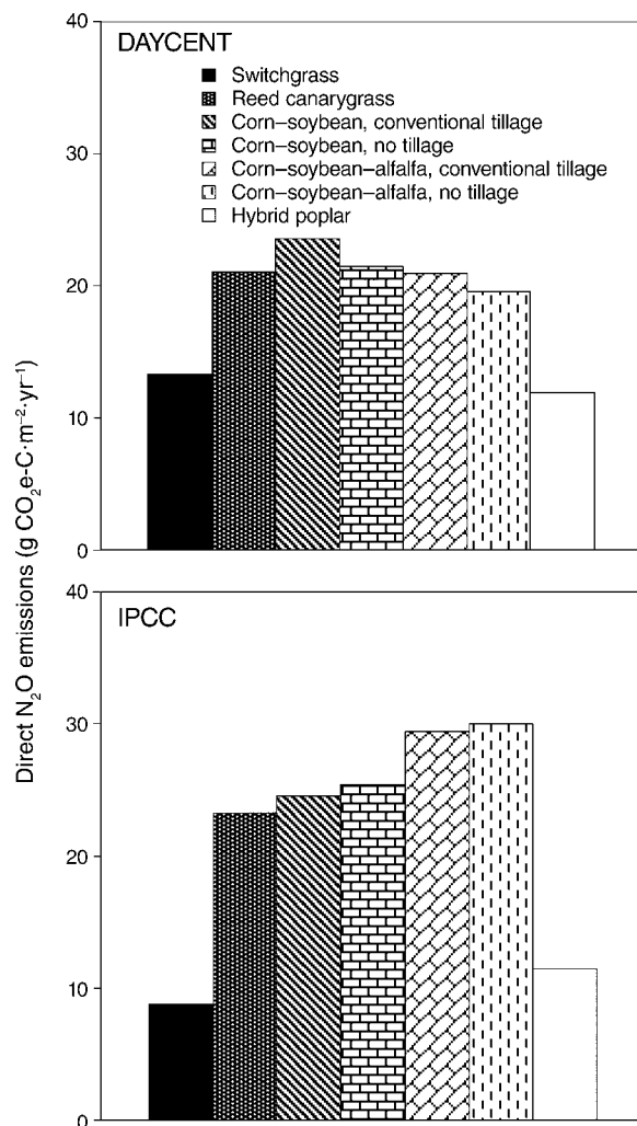
FIG. 3. Intergovernmental Panel on Climate Change (IPCC 2000) and DAYCENT (Del Grosso et al. 2001a) calculated direct N_2O emissions from bioenergy cropping systems.
