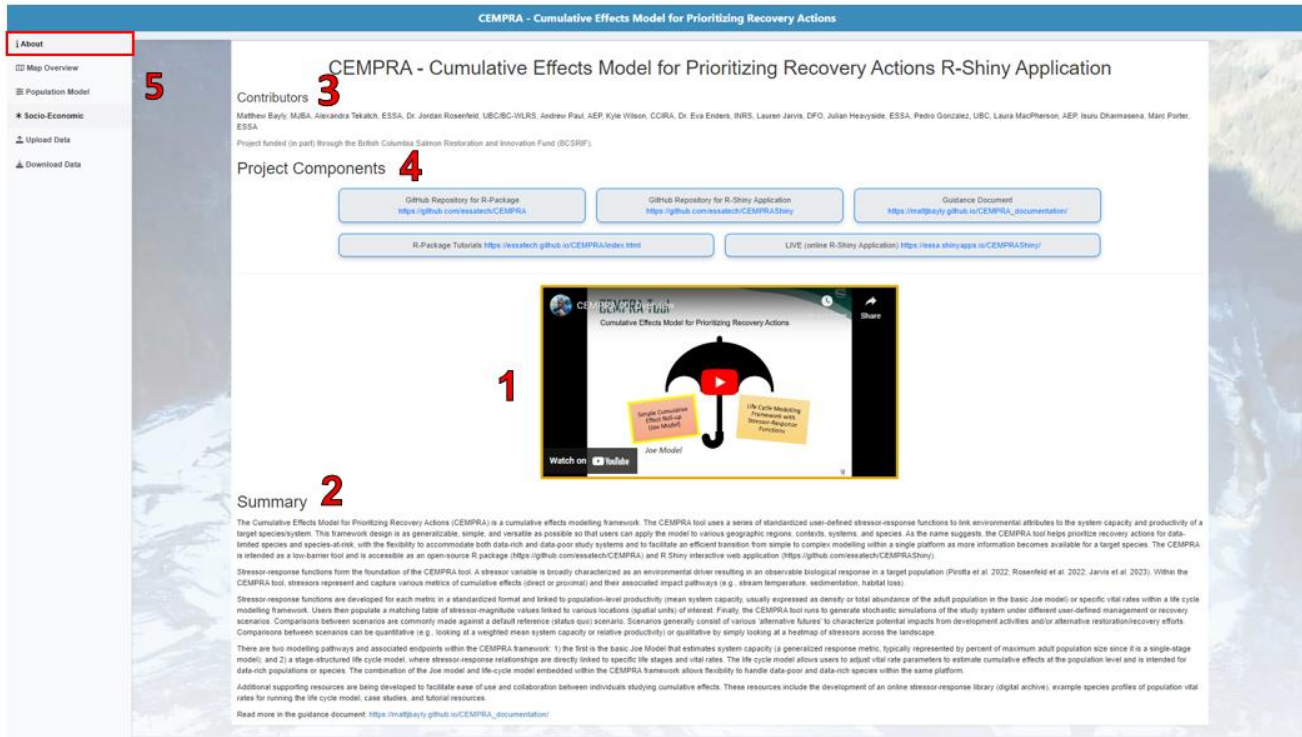
Figure 14. About page in the R Shiny web application. 1) Tutorial video for using the R Shiny application. 2) Brief introduction to the CEMPRA and associated life cycle model. 3) List of contributors to the CEMPRA. 4) List of components included in the CEMPRA project. 5) Menu for the R Shiny application.
