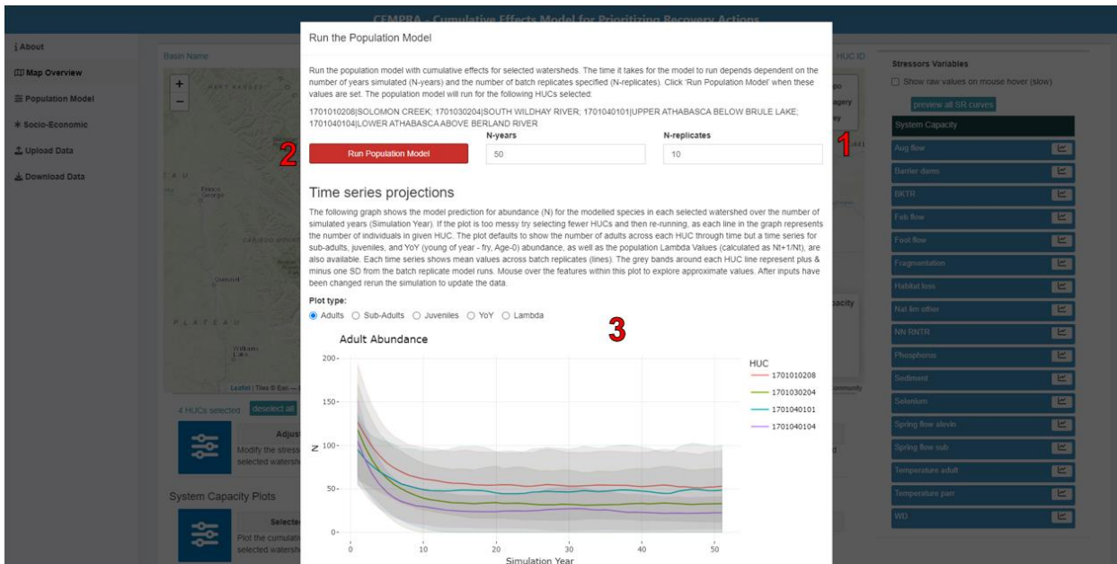
Figure 20: Pop-up window for the life cycle model. 1) Input boxes for the number of years and number of replicates in the simulation. 2) The button to run the life cycle model. 3) Plotting window for time series projection plots.
